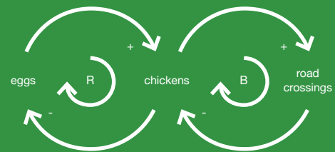
Dynamic complexity
