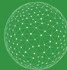
Dynamic complexity
